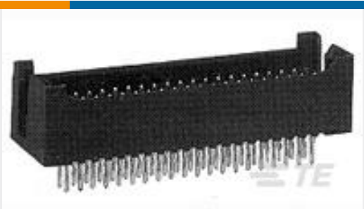
TE Part # 5-534245-4 16 MODII 2PC HDR DRRA W/HLDWN, ROHS
